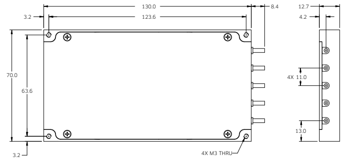
Dimensions Diagram (Specifications in mm unless otherwise noted.)
