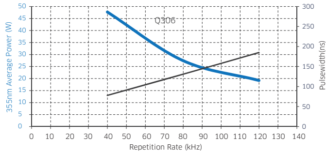
Figure 1. Q306 typical power and pulse width curve
