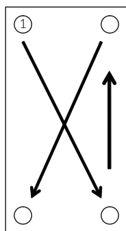
Initial torque to ~0.75 in-lb
