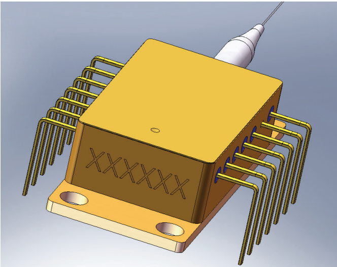
Figure 3b. Leads bent downwards 90 degrees
