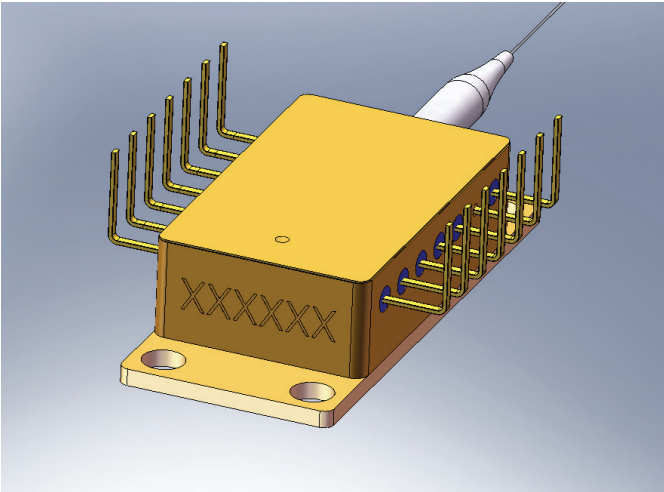
Figure 3a. Leads bent upwards 90 degrees
